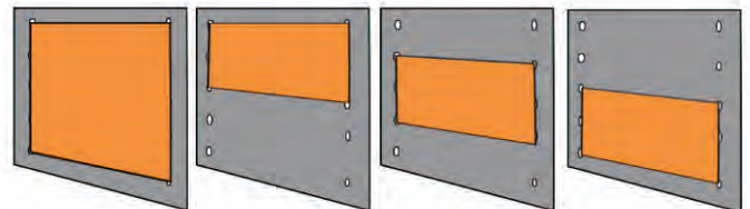
TC35FC and TC35FCFF features a VESA compliant mounting plate for monitors with a 200mm x 200mm or 200mm x 100mm mounting hole pattern
